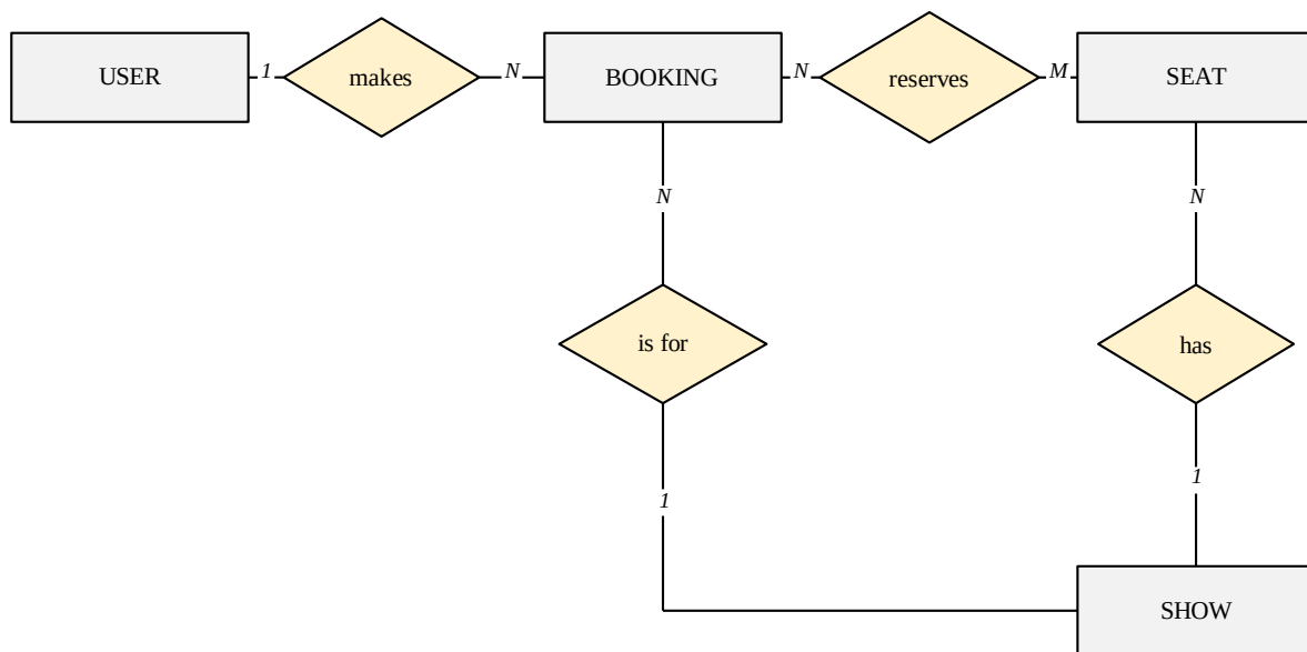
Figure 4.7 Conceptual entity relationship diagram
