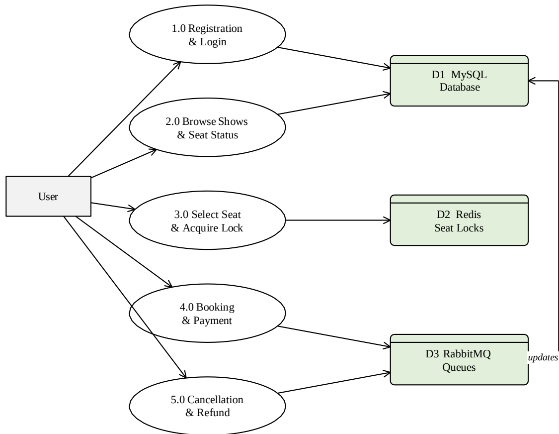
Figure 4.2 Level-1 Data Flow Diagram
