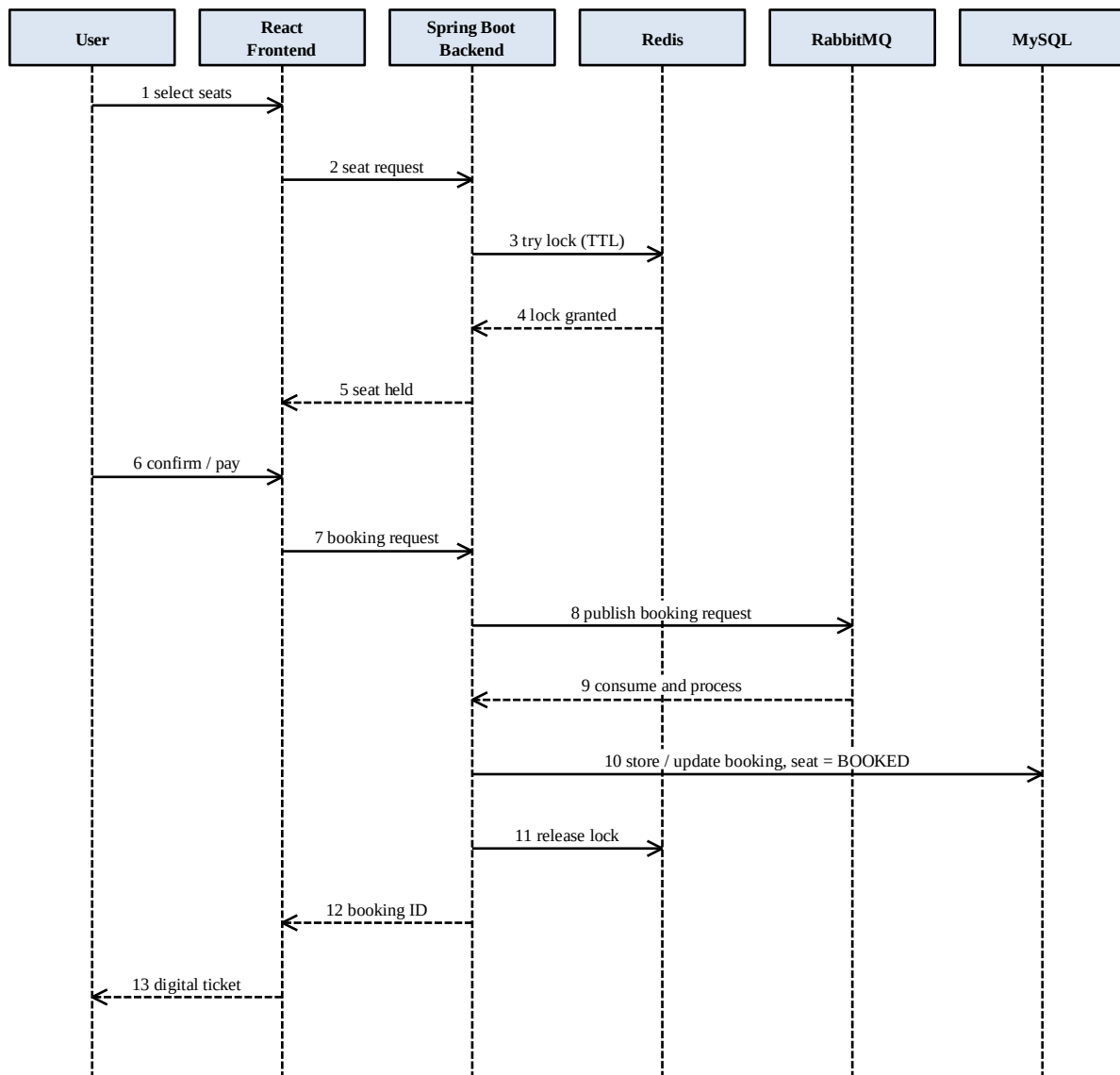
Figure 4.5 Sequence diagram of a successful booking
