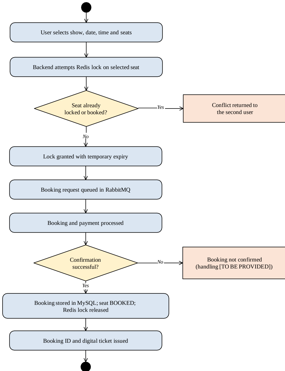
Figure 4.4 Activity diagram of the seat booking process
