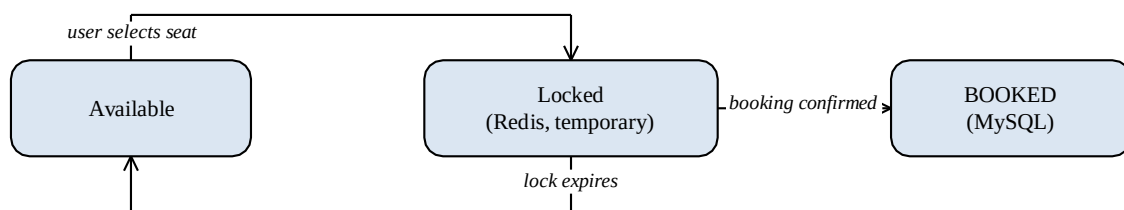
Figure 5.3 Seat states during the booking process
