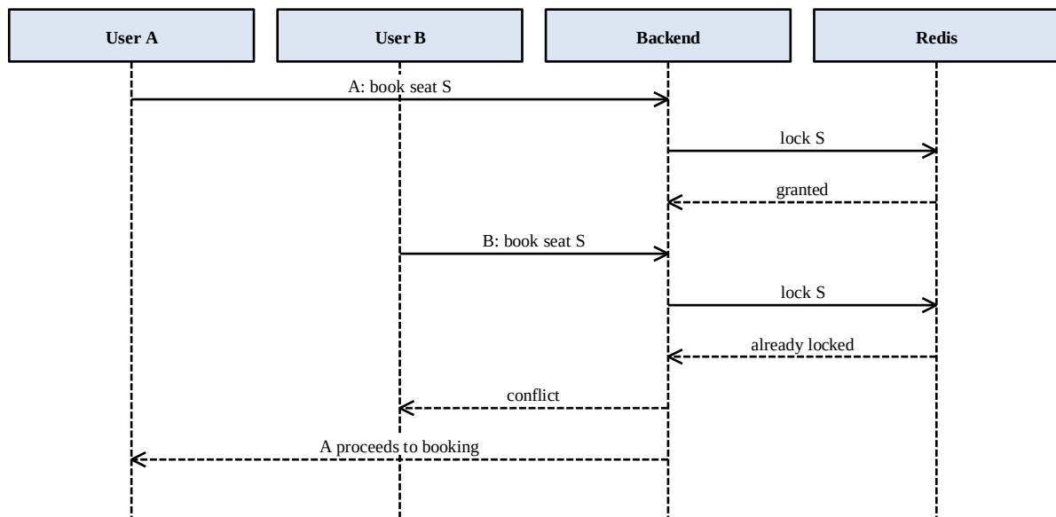
Figure 5.2 Two users attempting to book the same seat
