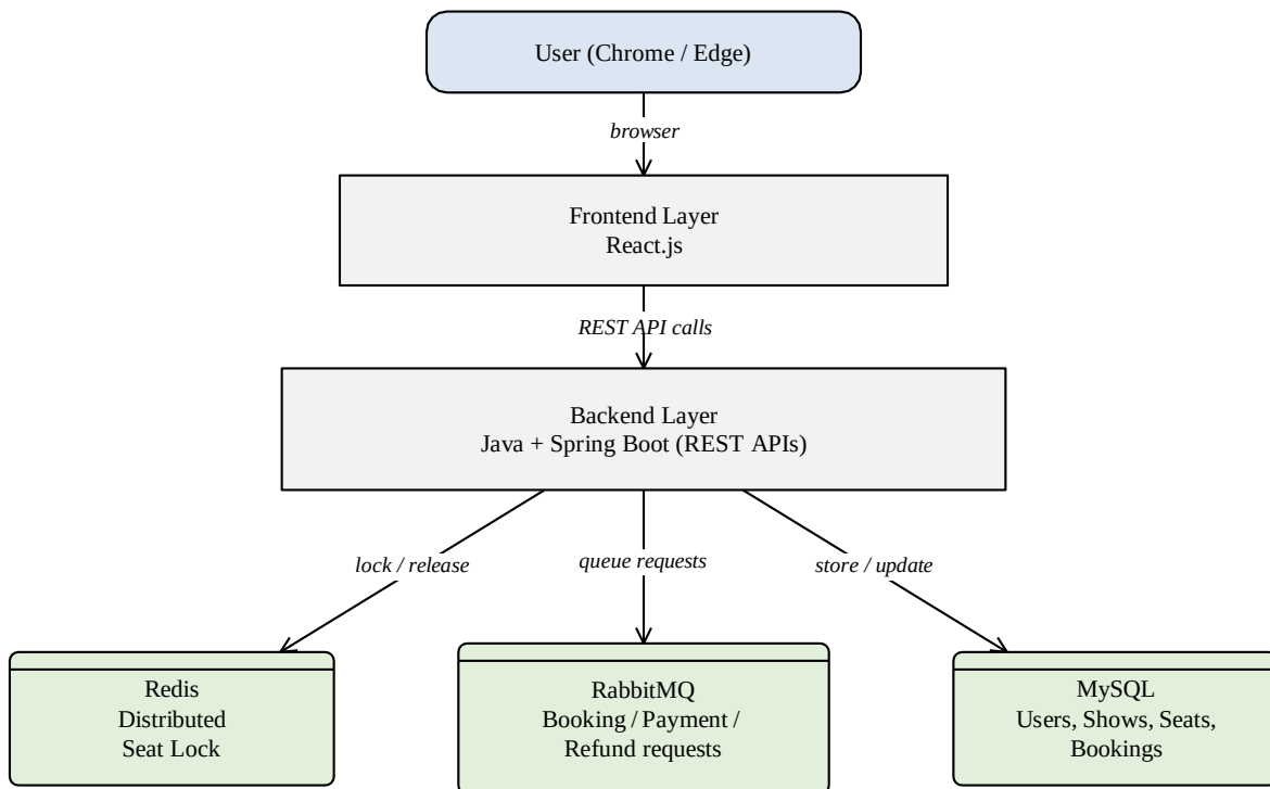
Figure 4.1 High-level architecture of the Ticket Booking System
