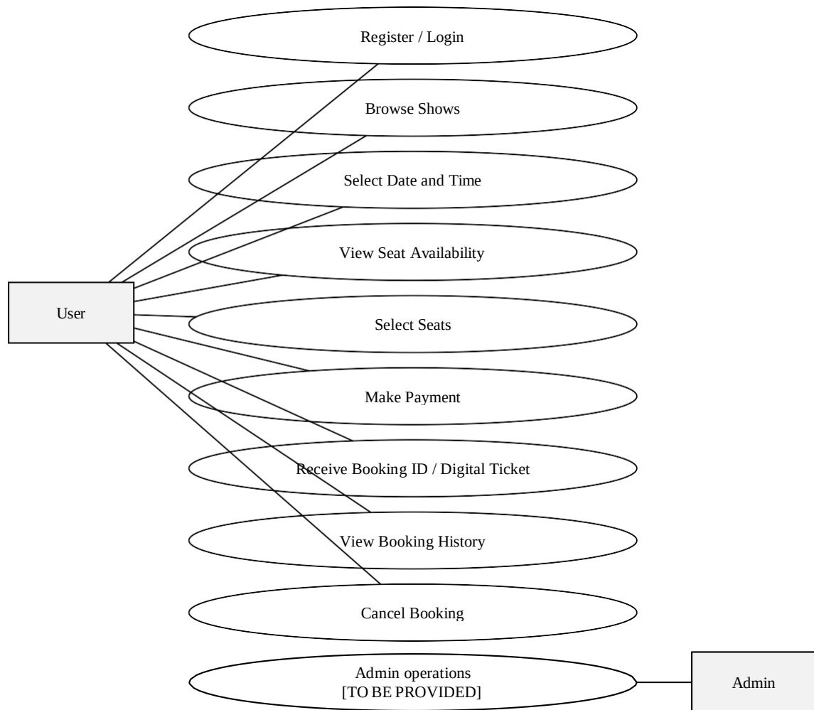
Figure 4.3 Use case diagram of the Ticket Booking System
