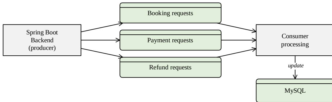
Figure 5.1 Queue processing through RabbitMQ (names of queues to be confirmed)
